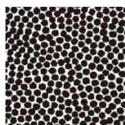
Conventional Pebble Surface Average texture top area @ 2.74mm 2
